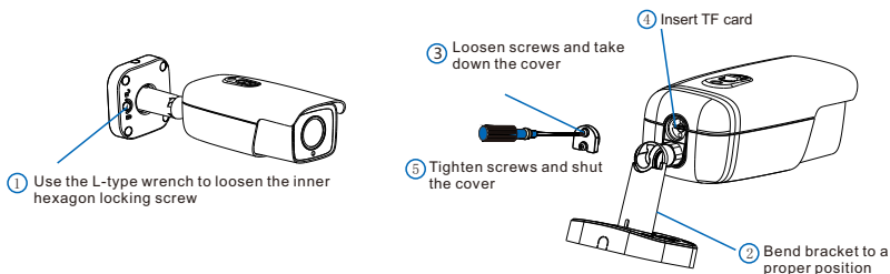
TF Card Installation of Models With A Bracket
