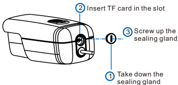
TF Card Installation of Models Without A Bracket
